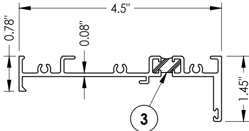
2 BLOCK FRAME
