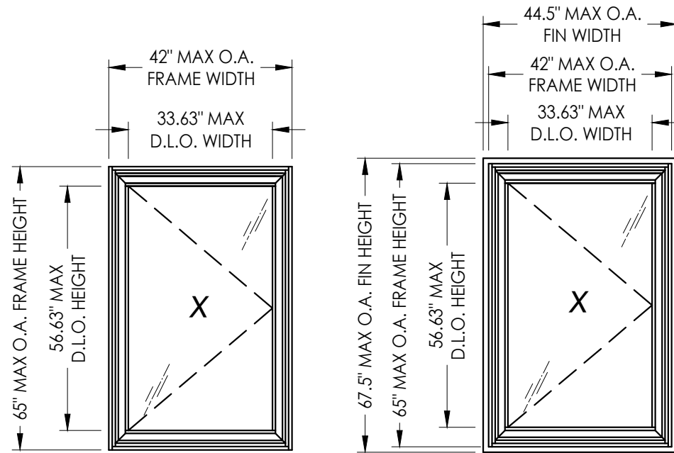
FRAME MOUNT
